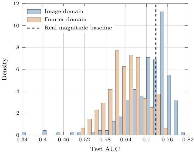
Figure 1: Distribution of test AUC across the 480 complex-valued configurations. Image-domain and Fourier-domain configurations are shown using identical histogram bins; the dashed vertical line denotes the fixed real magnitude baseline.
