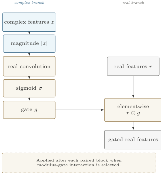
Figure 5. Implemented interaction mechanisms. The modulus gate derives a sigmoid gate from complex-feature magnitudes and applies it multiplicatively to the corresponding real-stream features after each paired block. Holographic attention operates only on the complex branch after the third pooled stage, combining Hermitian query–key similarity with a magnitude-distance penalty before complex value aggregation.
