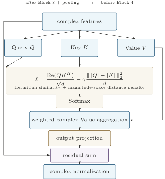
Figure 5. Implemented interaction mechanisms. The modulus gate derives a sigmoid gate from complex-feature magnitudes and applies it multiplicatively to the corresponding real-stream features after each paired block. Holographic attention operates only on the complex branch after the third pooled stage, combining Hermitian query–key similarity with a magnitude-distance penalty before complex value aggregation.
