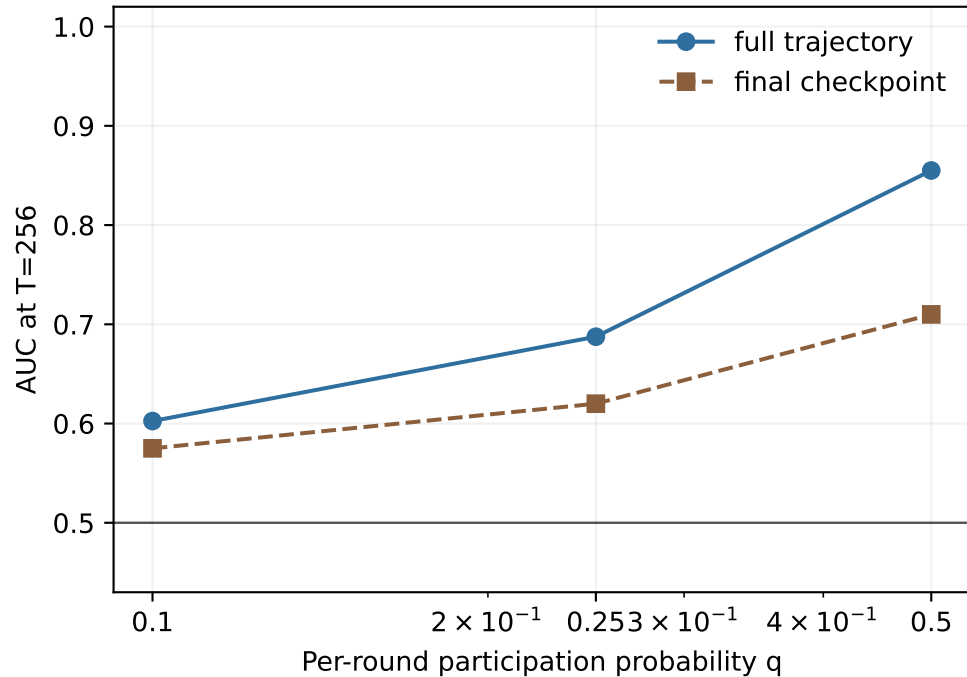
(b) Trajectory versus endpoint
