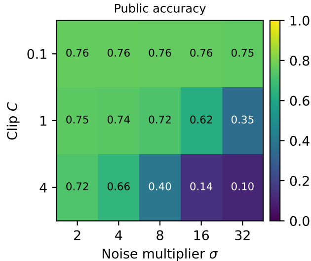
Matched clip/noise grid at T=64
