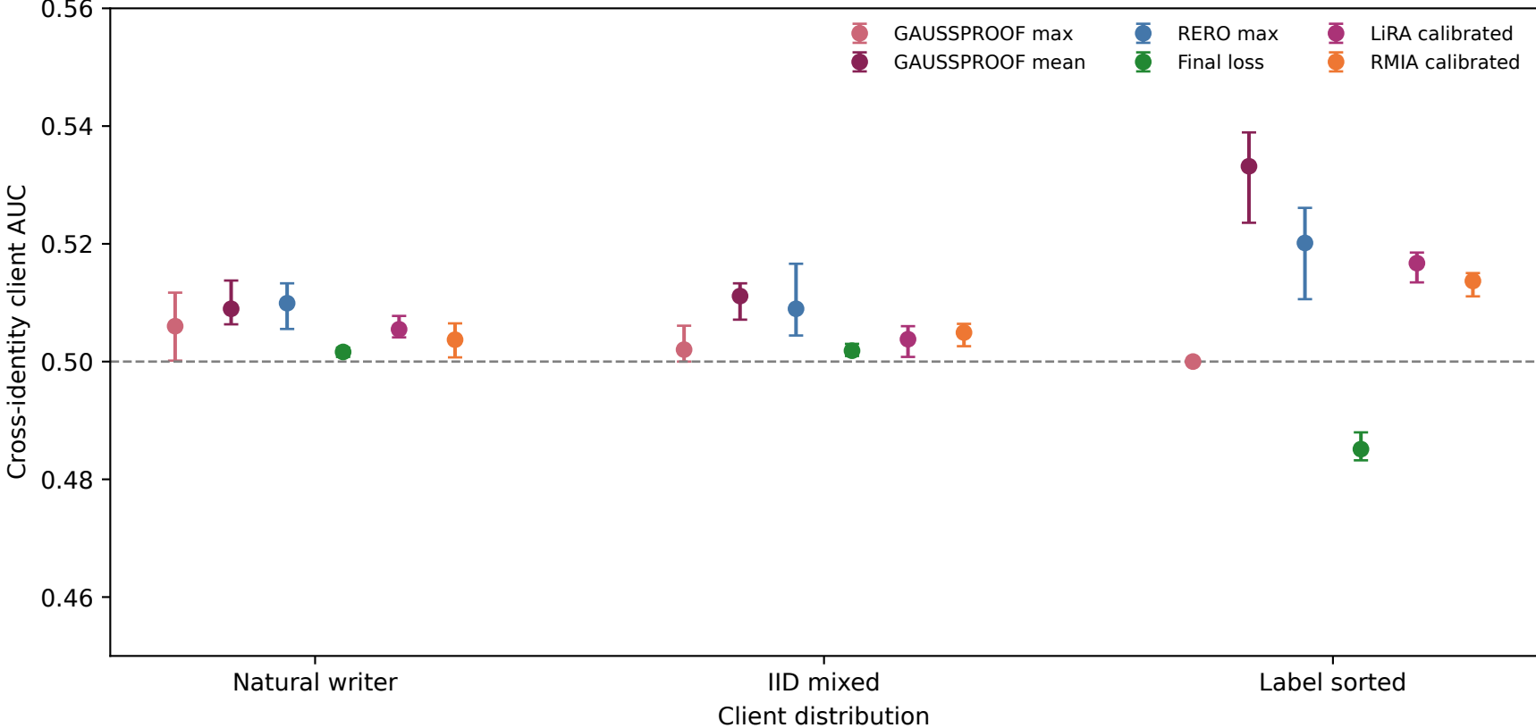
8 clients/round, \sigma=.25 (public attacks; zoomed AUC): mean and range over three seeds
