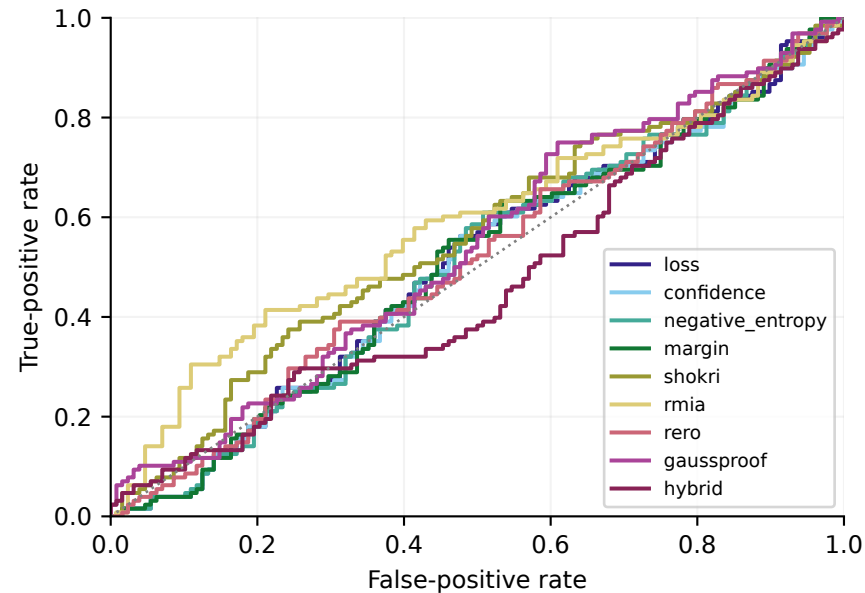
seed17_sigma0.5_clip1_B32
