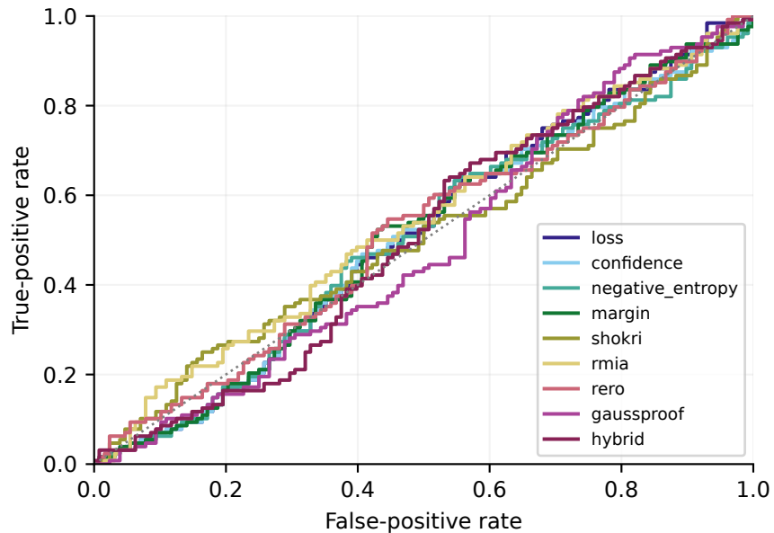
seed43_sigma0.5_clip1_B32
