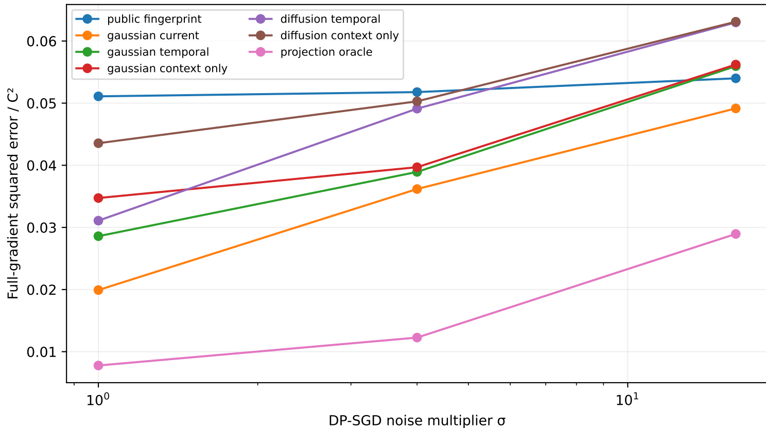
Evolving DP-SGD: causal clipped-average recovery
