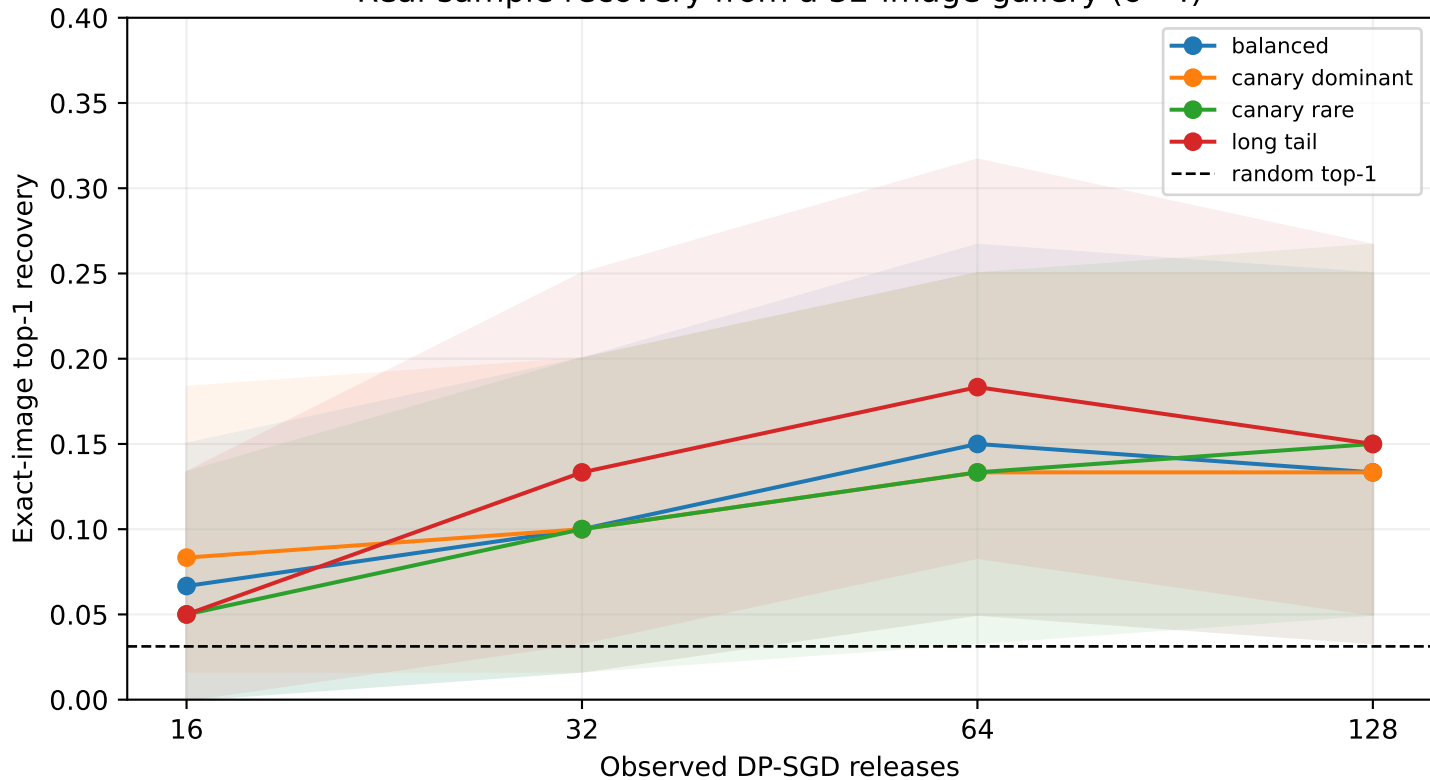
Real-sample recovery from a 32-image gallery ( \sigma=4 )
