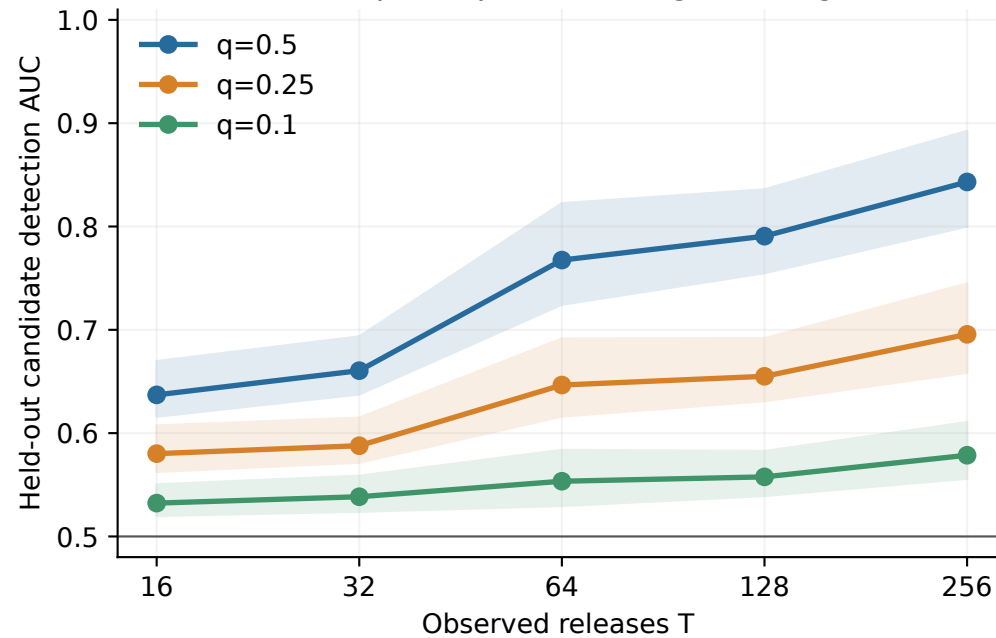
(a) More participation strengthens signal
