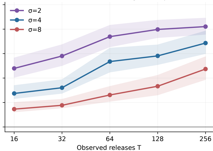
(b) More noise weakens signal at q=0.5
