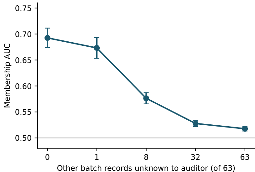
Background knowledge determines attack power
