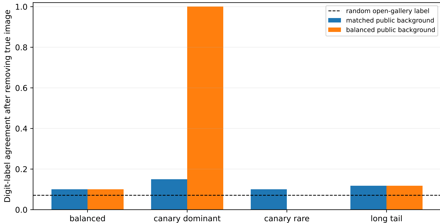
Class leakage under background-distribution mismatch
