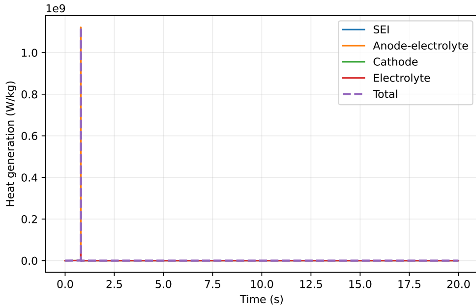
Figure 10: Mass-specific heat-generation rates associated with the thermal runaway reactions in the Hu et al. reference simulation.
