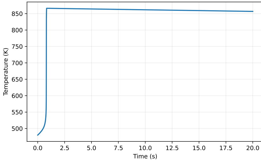
Figure 8: Cell temperature predicted by LiionTR for the Hu et al. reference thermal runaway simulation.
