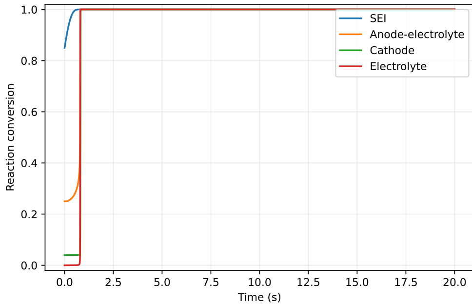
Figure 9: Evolution of the SEI, anode-electrolyte, cathode, and electrolyte reaction conversions during the reference simulation.
