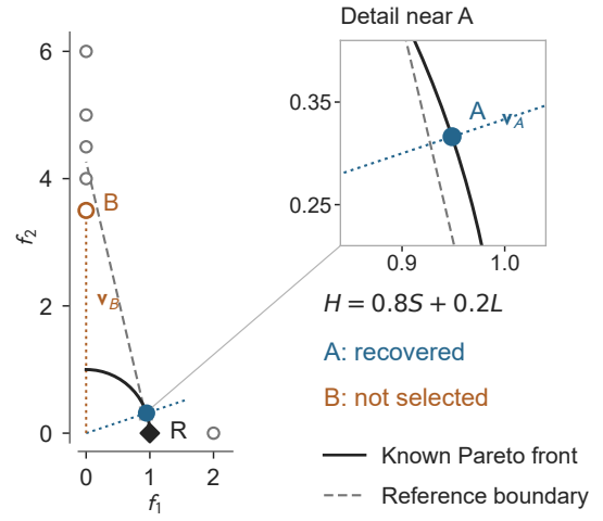
(b) Hybrid PBI ( t = 0.20 )
