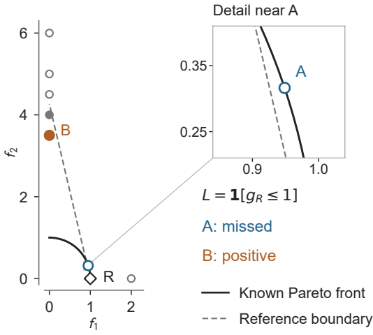
(a) Reference-solution PBI
