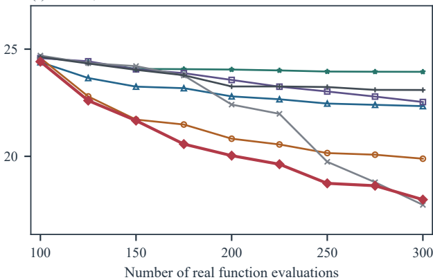
(f) WFG8, M = 20
