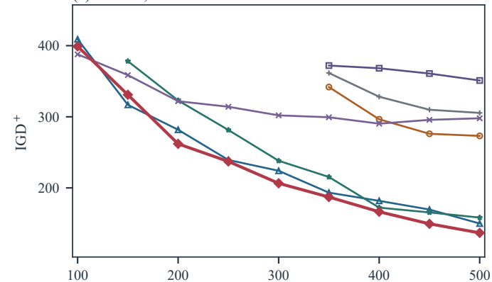
(a) DTLZ1, M = 10
