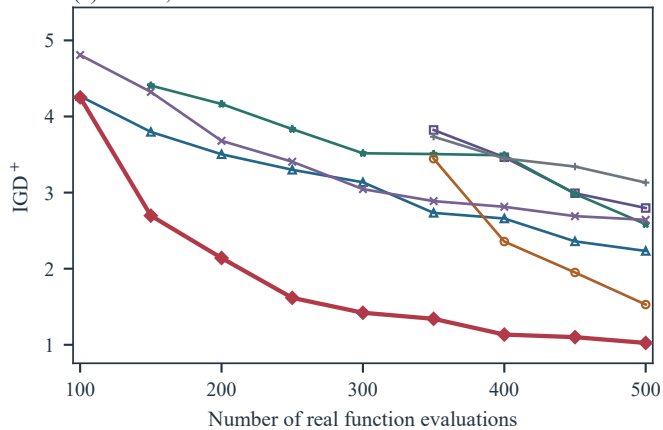
(c) WFG2, M = 10
