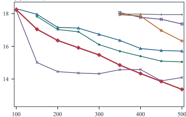
(b) DTLZ6, M = 10
