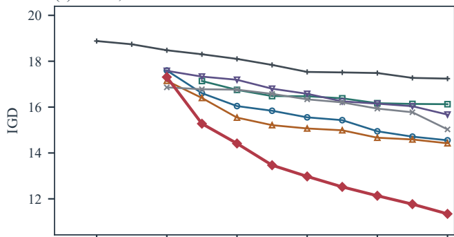
(c) WFG7, M = 15
