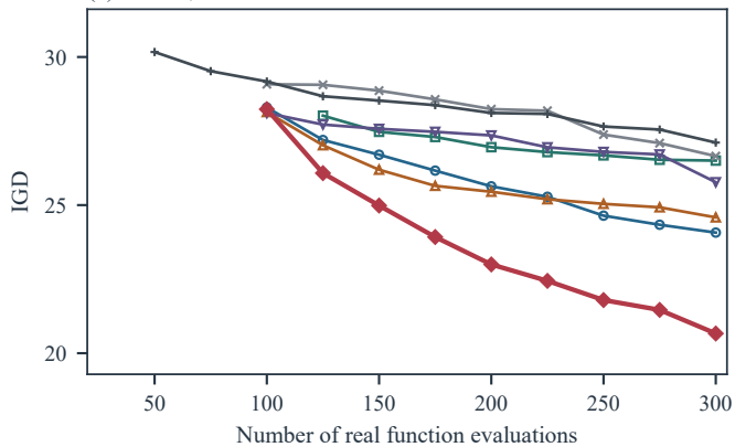
(e) WFG7, M = 20
