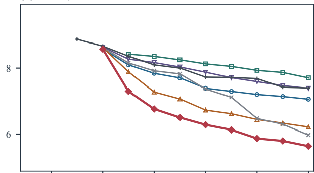
(b) WFG8, M = 10
