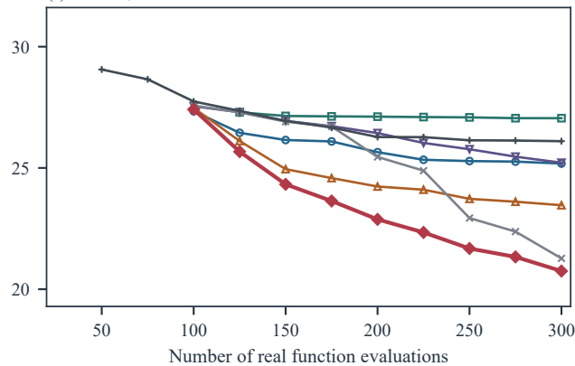
(f) WFG8, M = 20
