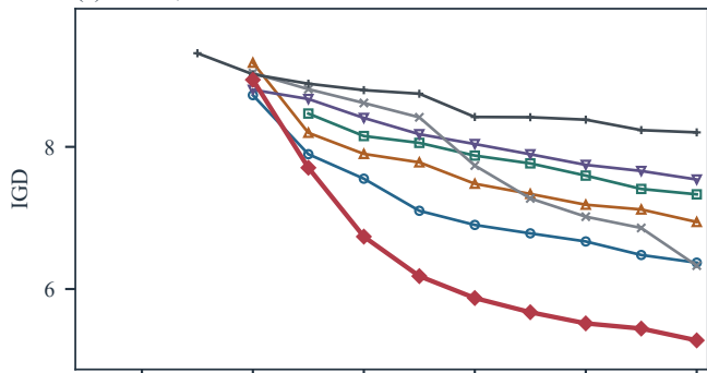
(a) WFG7, M = 10
