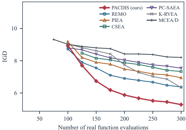
(a) WFG7, M = 10
