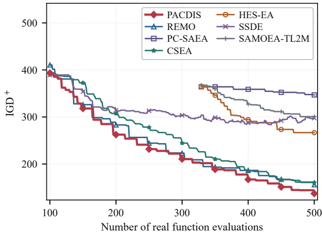
DTLZ1, M = 10
