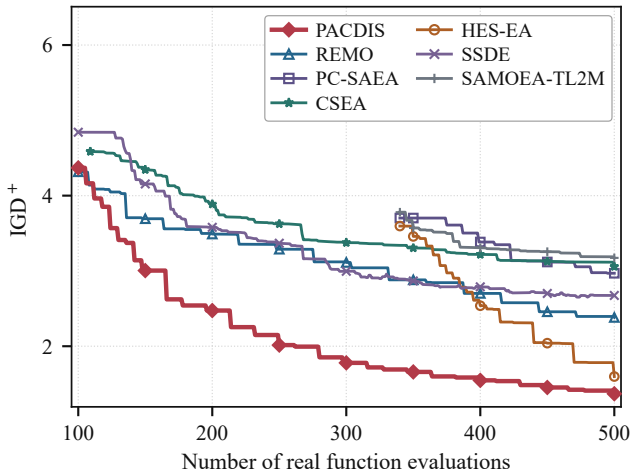
WFG2, M = 10
