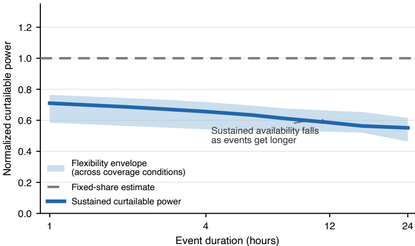
Normalized curtailable power versus event duration, by coverage level
