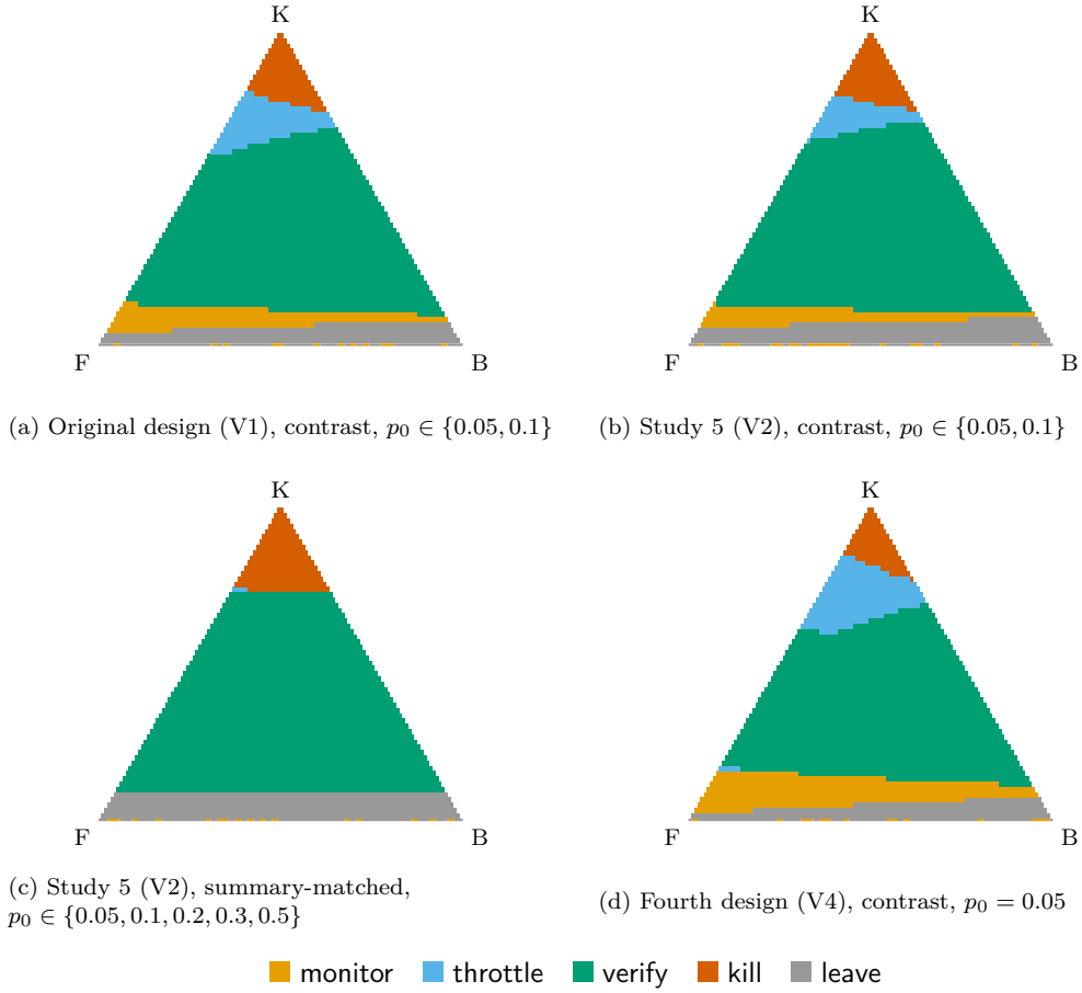
Figure 2: Optimal action on the simplex in the first period, before verification, at one representative three-state point of each cell (not the whole three-state set): K at the top, F bottom left, B bottom right. The benign shock's separation from the fault is a fraction 0.5 of d , a share 0.25 of the non-compromise prior mass is on B , \rho = 0 , \kappa = 0.5 , simplex grid N = 60 . Cells with identical maps share a panel.
