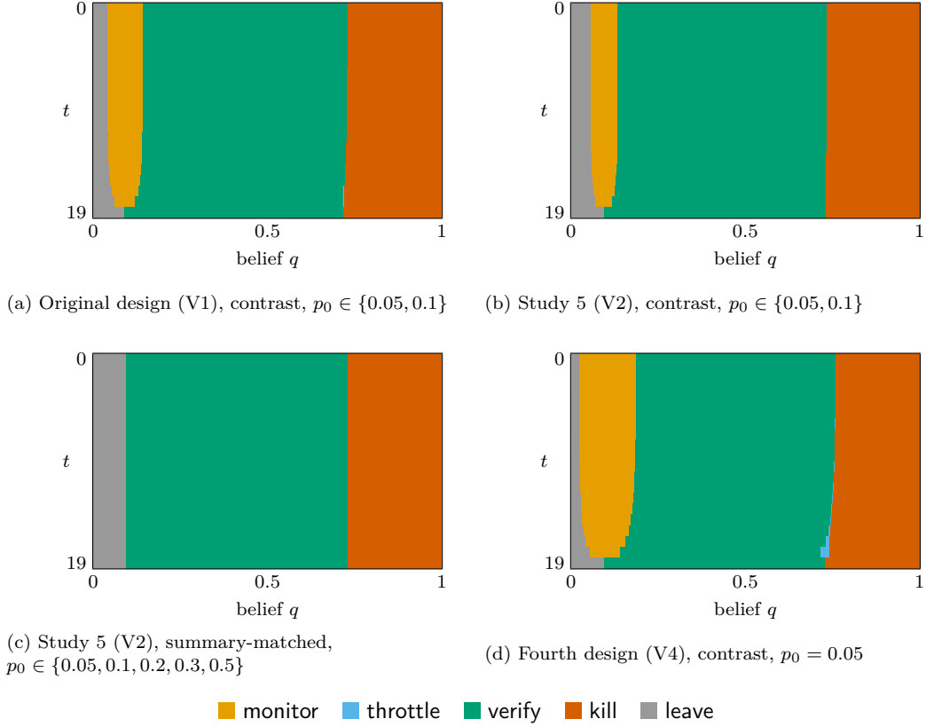
Figure 1: Optimal action over the belief q (horizontal) and the period t (vertical, t = 0 at the top) before verification, at one representative point of each cell of \mathcal{F} : n_W = 4 , \eta = 1 , \rho = 0.25 , \zeta = 0.1 , \kappa = 0.5 , s = 0.9 , t_F = 0.9 , horizon T = 20 , belief grid of 401 points. Cells with identical maps share a panel.
