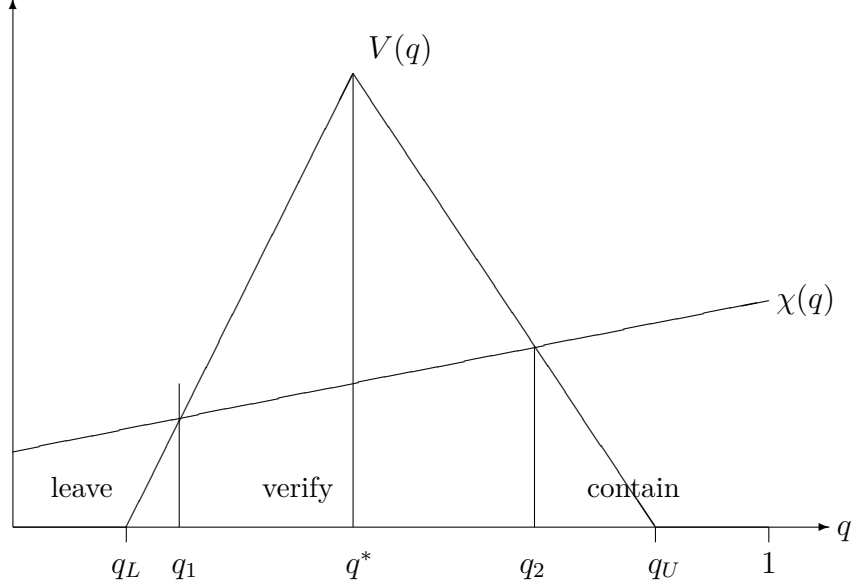
Figure 1: Schematic of Lemma 3 and Theorem 1 (not to scale; no parameter values; critical delays for the checks of the empirical study are in Table 7). The value of information V is a tent on (q_L, q_U) with its peak at the passive threshold q^* ; the verification cost \chi increases with the belief because harm during the delay accrues only under compromise. Verification pays on (q_1, q_2) , where the tent lies above the cost line. Raising the delay \tau tilts the cost line upward and shrinks the interval (Theorem 2).
