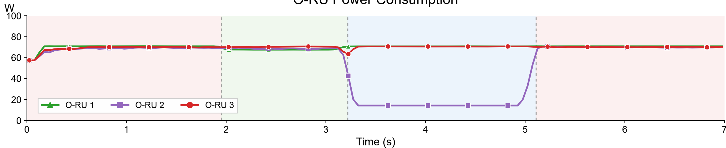
O-RU Power Consumption
