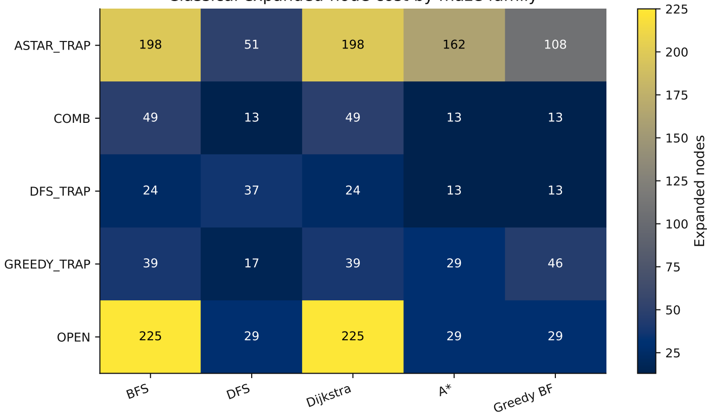
Classical expanded-node cost by maze family
