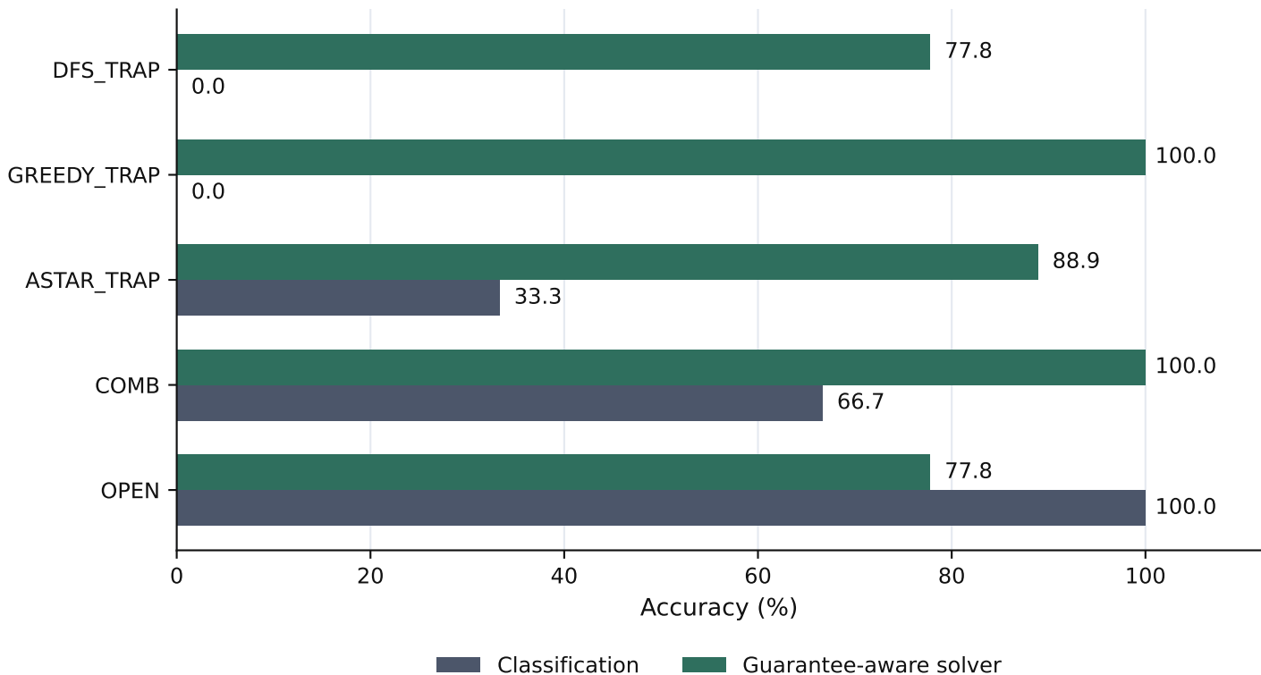
Solver recommendation can succeed when classification fails
