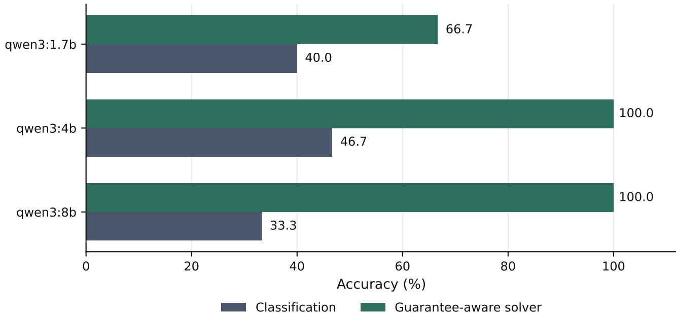
Prompt v3 performance by local model
