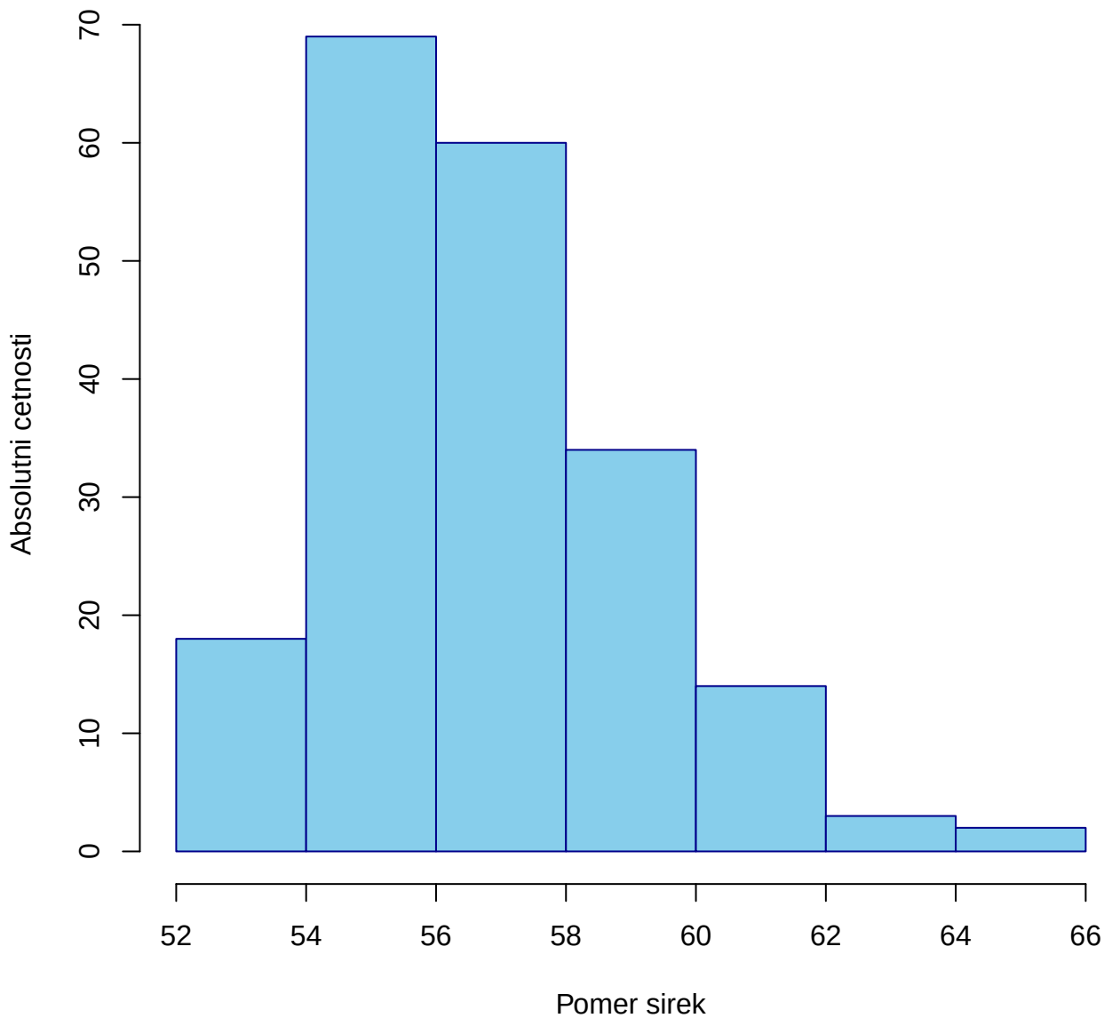
Histogram
