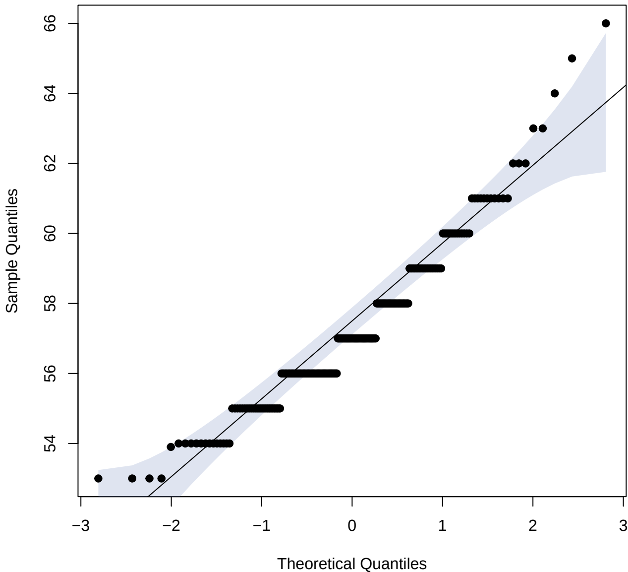
Q-Q-Plot (qnorm)
