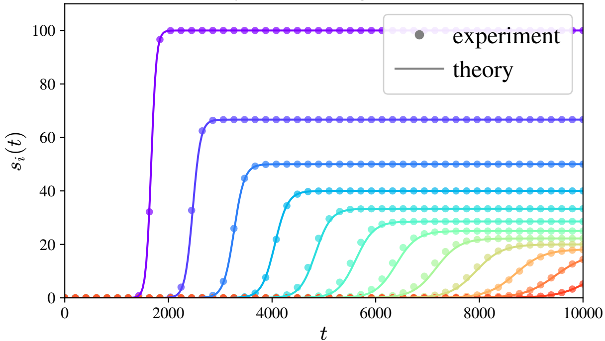
Gradient flow dynamics of singular values of W_2W_1
