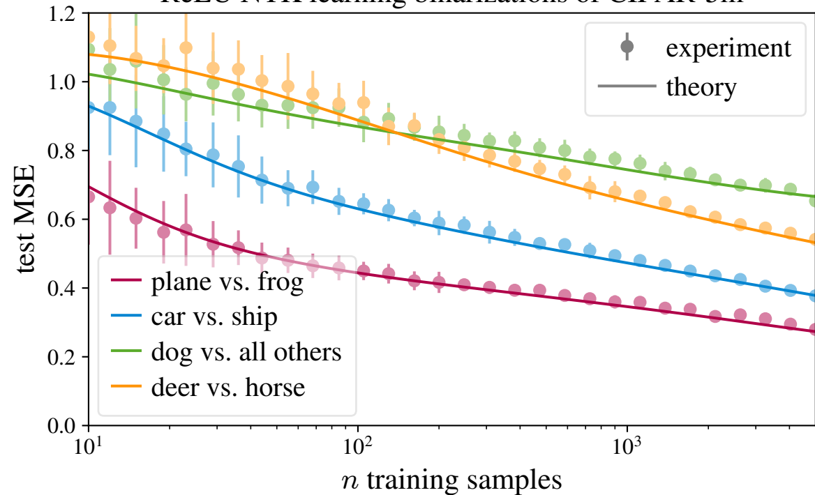
ReLU NTK learning binarizations of CIFAR-5m
