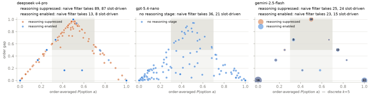
Figure 1: Order-averaged P(\text{option a}) against order gap, one point per pair per setting, on the two targets whose APIs expose log-probabilities. The shaded column is what a naive 0.3–0.7 split filter accepts; the darker block is the part of it that is position-driven. Perfect balance and total position dependence coincide at the apex, and the same structure appears on gpt-5.4-nano , which has no reasoning stage to disable — so the shape is not an artefact of suppressing reasoning. gemini-2.5-flash is absent because that API returns no log-probabilities and the discrete estimate at k = 5 is too coarse to resolve the shape; its order gap is in Appendix D.
