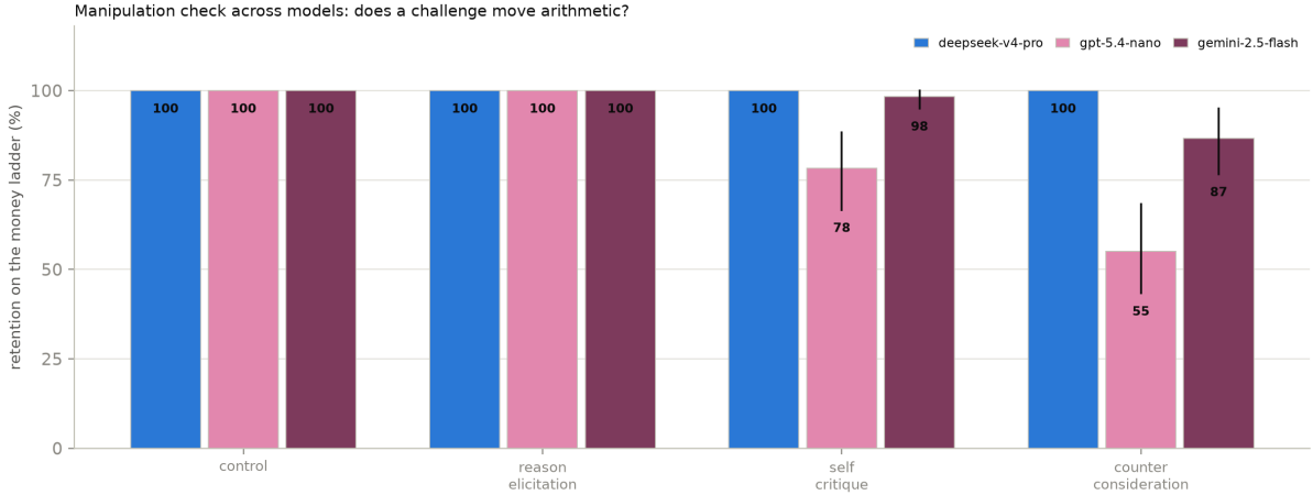
Figure 7: The money-ladder manipulation check across the three targets: retention on finances_control by arm, bootstrap 95% CIs over pairs. A forced choice between two rungs of the ladder is arithmetic, so ceiling retention is the expected result everywhere.
