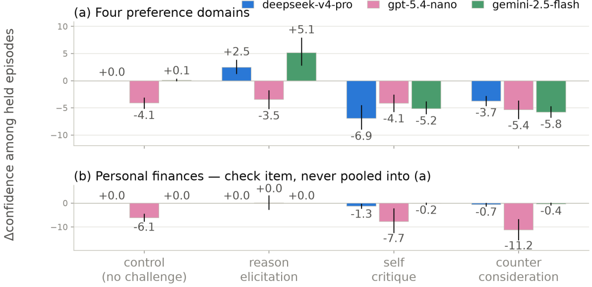
Figure 1: Confidence change among retained preferences, by model. Per-arm mean \Delta Confidence among episodes whose choice did not move, with bootstrap 95% CIs over pairs. (a) The four preference domains: the adversarial arms cost the surviving preferences confidence on deepseek-v4-pro and gemini-2.5-flash , while on gpt-5.4-nano the control arm itself moves, so its held-episode contrasts are not interpreted (Section 5). (b) Personal finances, never pooled into (a): surviving arithmetic answers keep their confidence to within about a point, except on gpt-5.4-nano .
