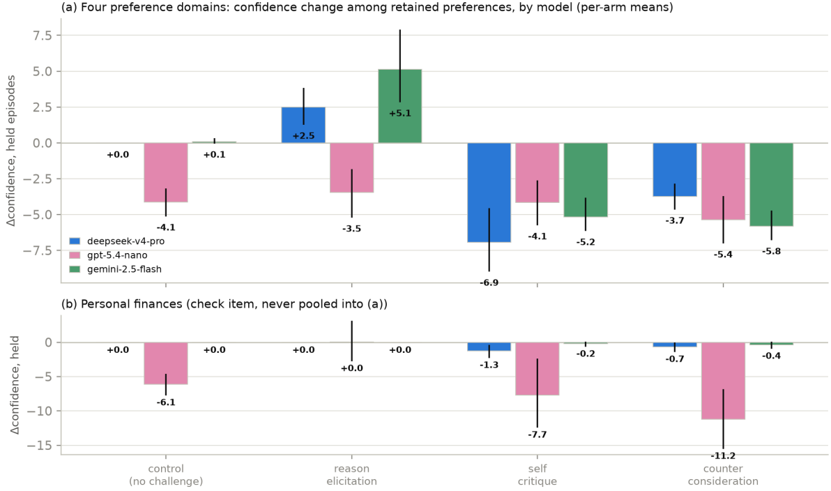
Figure 3: Figure 3: Confidence change among retained preferences, by model, all five approved domains. Per-arm mean \Delta Confidence among episodes whose choice did not move, with bootstrap 95% CIs over pairs. (a) The four preference domains: on deepseek-v4-pro and gemini-2.5-flash the two adversarial arms cost the surviving preferences confidence while control sits at or near zero; on gpt-5.4-nano the control arm itself moves, so its held-episode contrasts are not interpreted (Section 5). (b) Personal finances, never pooled into (a): on deepseek-v4-pro and gemini-2.5-flash the surviving arithmetic answers keep their confidence to within about a point, while gpt-5.4-nano loses confidence even on arithmetic — including under its moving control.
