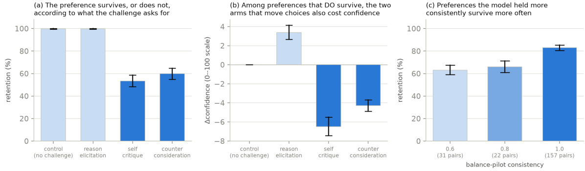
Figure 6: Persistence under challenge over the combined set — the original run and the five-domain extension together, 2520 scored episodes across the 8 preference domains, 210 pairs on deepseek-v4-pro. Bars are means, whiskers bootstrap 95% CIs over pairs. finances_control is a positive control rather than a domain and is held out of all three panels (240 episodes); it is reported on its own in Section 4.3. (a) Retention by arm. (b) \Delta confidence among episodes that held , not differenced against control — control sits at zero. The held-episode figures quoted in Section 4.2 are the original-domain estimates and are slightly smaller than the pooled ones shown here; the difference is which domains are included, not a disagreement. (c) PQ2: retention against balance-pilot consistency, which at k = 5 takes three values.
