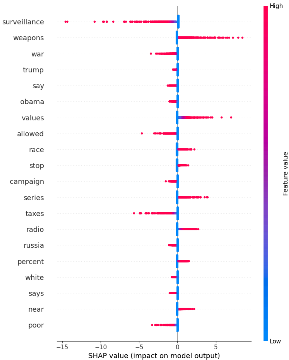
Figure 4: Global Feature Importance and Impact Analysis of Logistic Regression
