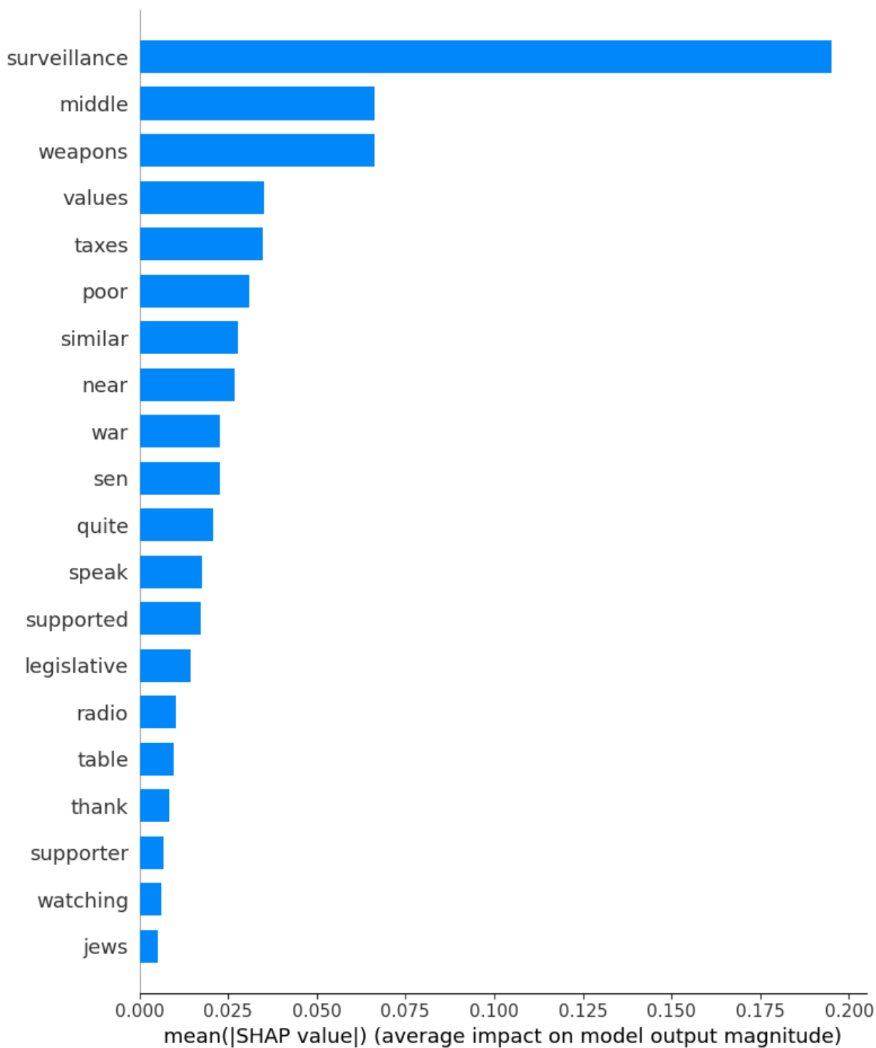
Figure 7: Mean absolute SHAP values across 80 samples (bottom)
