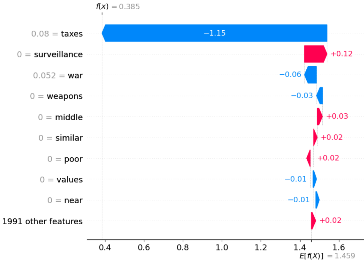
Figure 5: SHAP Waterfall force plot for a representative sample
