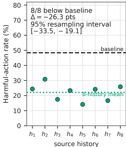
A. Qwen3-30B consistent within panel
