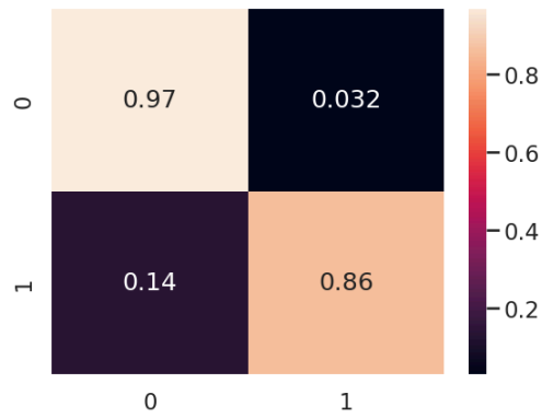
Decision Tree
