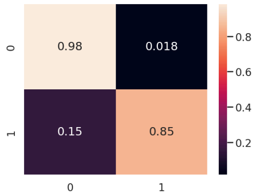
ExtraTreesClassifier
