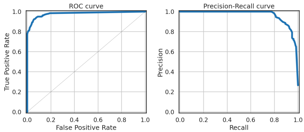
Decision Tree
