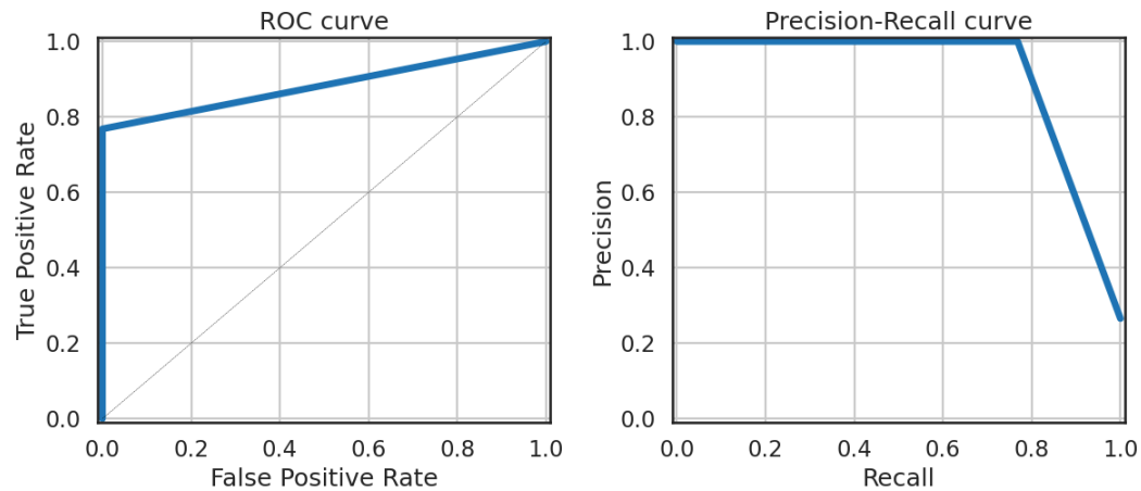
Stacked
