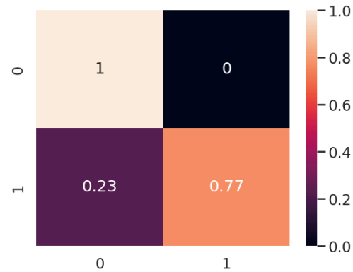
AdaBoost Classifier
