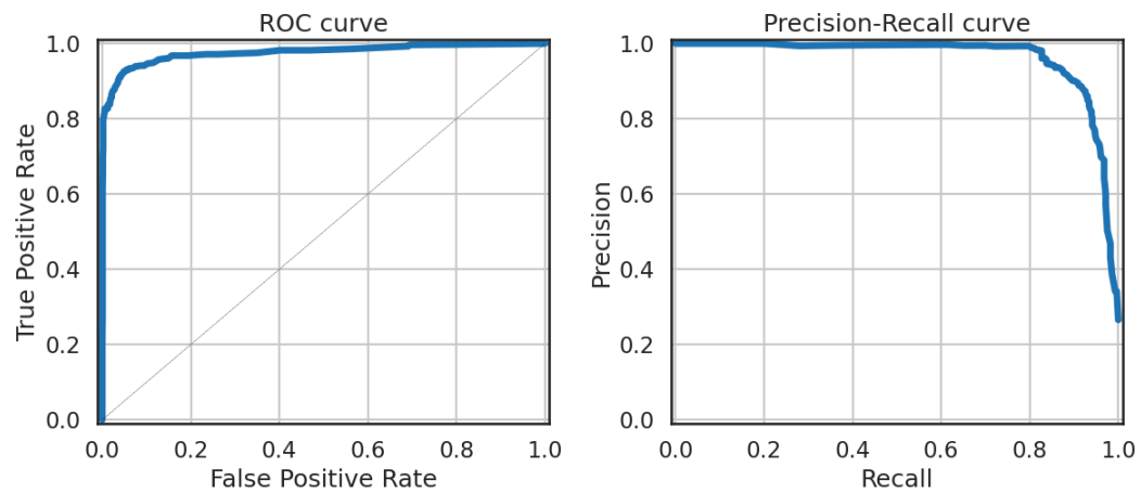
ExtraTreesClassifier
