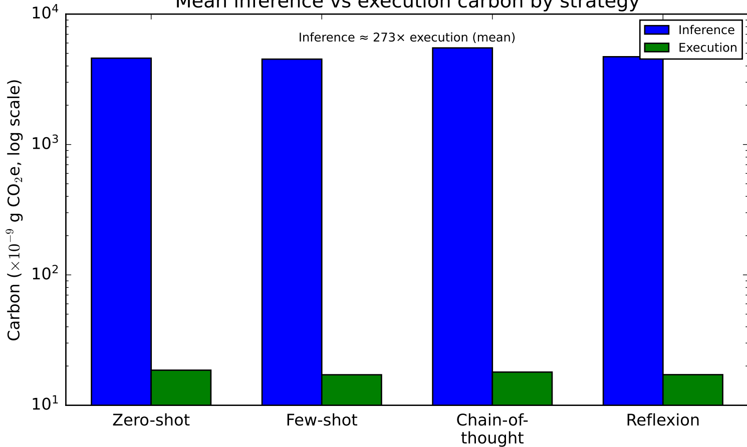
Mean inference vs execution carbon by strategy
