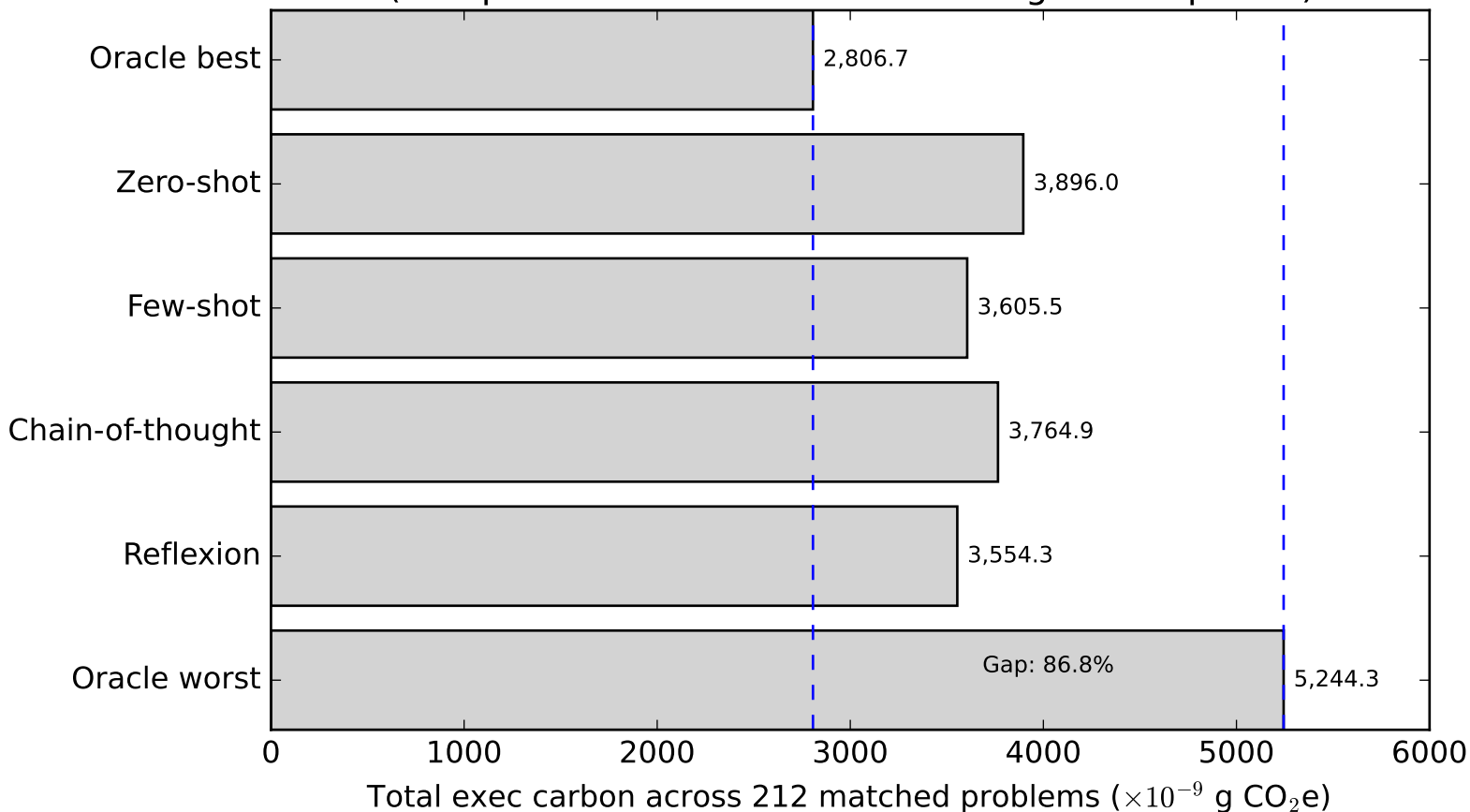
Oracle best / worst vs fixed strategy totals (212 problems where all four strategies completed)
