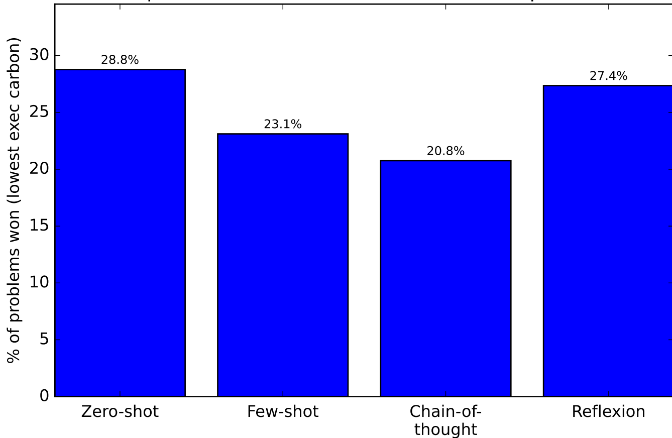
Per-problem win rates across 212 matched problems
