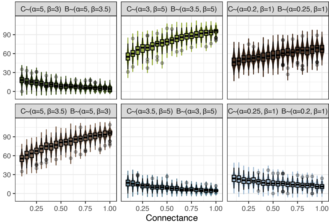
Distribution of surviving species
