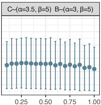
Connectance
