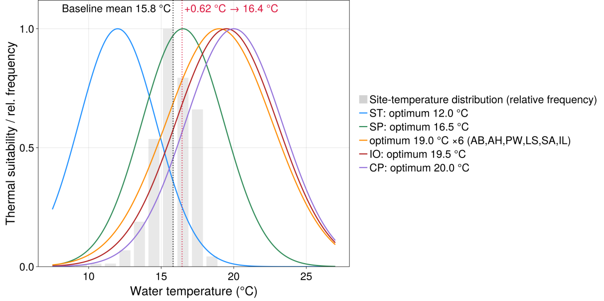
Figure 1: Thermal niches against baseline water temperature. Grey bars: relative frequency of the 2026 baseline water temperature across all 775 sampling sites (1 °C bins, normalised to the tallest bar). Coloured curves: the Gaussian thermal-suitability function W = \exp[-(T - T_s^*)^2 / (2\sigma_s^2)] for the native species; species with identical empirical ranges are drawn once. In the legend, which is placed outside the plotting area, each colour gives a species code and its optimum T_s^* , using the same species grouping convention as Fig. 2. Because \sigma_s is one-sixth of the empirical range, suitability falls to \exp(-9/2) \approx 0.011 at the range edges. Vertical lines: dotted black is the corrected basin-mean baseline temperature (15.82 °C); dotted crimson is the ensemble-median warming to 2045 on the corrected realised-forcing axis. Reading: the dominant cyprinids peak at 19–20 °C, warm of the present mean, so modest warming moves them towards their optima, whereas brown trout ( Salmo trutta , ST, optimum 12.0 °C) has a mean baseline of 13.72 °C at its 72 baseline-established sites, about 0.65 thermal standard deviations above its optimum.
