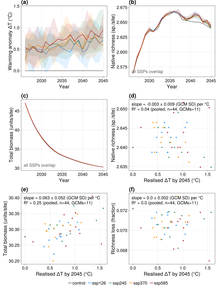
Figure 5: Forcing versus response in the corrected climate ensemble. “Forcing” is the realised basin-mean water-temperature anomaly \Delta T relative to the 1986–2005 baseline. Panels (a)–(c), annual trajectories 2026–2045: (a) forcing \Delta T ( ^{\circ}\text{C} ); (b) native richness (species per site); (c) total biomass (model units per site). Each line is the median across the 11 GCMs for one SSP pathway and the shaded band is the 10–90% range across GCMs; colours are blue = SSP1-2.6, green = SSP2-4.5, orange = SSP3-7.0 and red = SSP5-8.5. The native-richness and biomass panels overlap so closely that the in-panel annotation “all SSPs overlap” flags that the response trajectories lie on top of one another even though the forcing separates. Panels (d)–(f), end-of-2045 responses, one point per GCM \times SSP run (44 scenario runs): (d) end-of-2045 native richness; (e) end-of-2045 total biomass; (f) end-of-2045 realised richness loss; each is plotted against the realised warming of that run, with points coloured by SSP and the pooled ordinary-least-squares slope, GCM standard deviation and R^2 annotated in the panel. The realised anomaly is used because it is the quantity that drives the biology in each run (correction C7). Correlations are computed across the 44 scenario runs; the no-warming control is plotted for reference but excluded from the fits, matching the dose–response analysis. The loss metric is a deterministic thresholded realised loss, not an extinction probability. Reading: warming separates the pathways in panel (a), but the aggregate richness, biomass and loss responses remain nearly coincident across pathways over this horizon.
