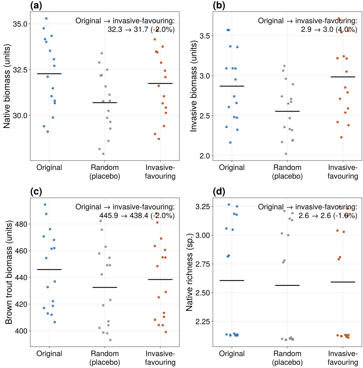
Figure 14: Interaction-matrix main effects. Panels: (a) basin native biomass; (b) basin invasive biomass; (c) brown trout final biomass; (d) basin native richness. x-axis: the three interaction assumptions (original, random placebo, invasive-favouring). Points: every one of the 16 runs per matrix (two climate endpoints \times two upstream costs \times four passability states), with slight horizontal jitter; the black horizontal line is the matrix mean. Annotations: the mean original \rightarrow invasive-favouring change. Relative to the original matrix the invasive-favouring matrix changed native biomass by -1.6\% , invasive biomass by +4.0\% , trout biomass by -1.7\% and native richness by -0.5\% , while total biomass changed by -1.2\% . These magnitudes are far smaller than the September bounding contrast and reflect the corrected interaction direction and the competitive Lotka–Volterra form; the sweep remains a bounding structural perturbation rather than a forecast.
