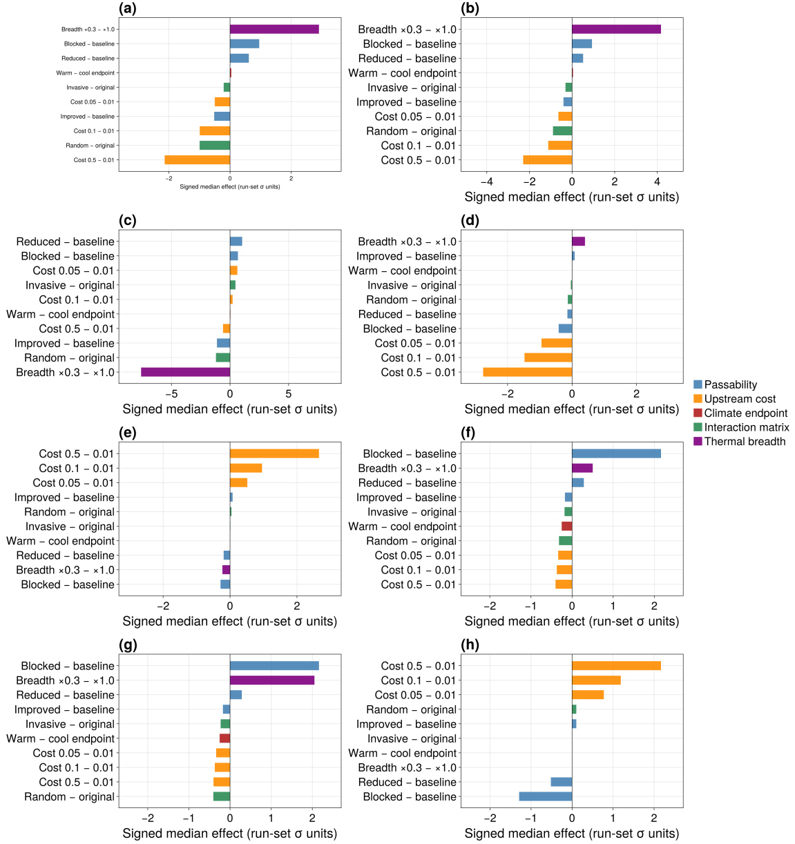
Figure 8: Signed factor effects (tornado), one panel per response metric. Panels: (a) total biomass, (b) native biomass, (c) invasive biomass, (d) native richness, (e) realised native richness loss, (f) brown-trout relative biomass change, (g) brown-trout final biomass and (h) brown-trout quasi-extinct fraction. Axes: the x-axis is the signed median effect in run-set standard-deviation ( \sigma ) units and a vertical black line marks zero, so a bar extending left means the level lowers the metric; the y-axis lists the factor levels being contrasted against their reference. Each bar: the median over matched factorial blocks of the signed difference between one factor level and its reference level, divided by the run-set standard deviation of that metric, so all bars are in comparable \sigma units. Bars are coloured by factor; the factor legend printed beside the panels defines the colours (passability, upstream cost, climate endpoint, interaction matrix and thermal breadth). Reference levels are upstream cost 0.01, baseline passability and the cool climate endpoint; the interaction-matrix and thermal-breadth contrasts are rescaled onto the main sweep's \sigma because the thermal-breadth multiplier is confounded with the sweep. Reading: increasing upstream cost reduces biomass and richness; blocked passability raises basin native and total biomass at every cost, while improved passability lowers it; and passability dominates trout biomass, consistent with the sum-of-squares results.
