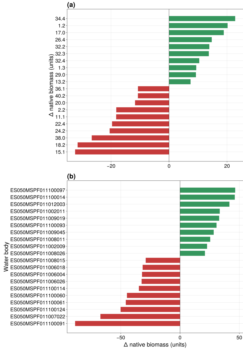
Figure 12: Spatial distribution of blockage effects. Scenario: warm endpoint, high upstream cost (0.50), end of 2045; blocked minus baseline passability. Panel (a): the 10 most negative and 10 most positive of the 77 sub-catchments. Panel (b): the 10 most negative and 10 most positive of the 289 water bodies. Both panels use the same x-axis (change in native biomass, model units) and show bars sorted from most negative to most positive; red bars are losses and green bars gains. The positive basin-level blocked-minus-baseline effect is a net of local gains and losses, so it must not be read as a uniform benefit of blocking; the sub-catchment or water body is the appropriate scale for management decisions.
