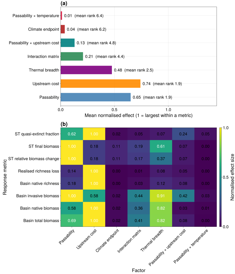
Figure 7: Factor importance in the corrected obstacle sweep. Panel (a): horizontal bars rank the seven factors of the sweep by their mean rank (1 = strongest; ties are broken by the plotting code’s factor order); the x-axis is the mean normalised effect across the eight response metrics (1.0 = the largest effect for that metric), each bar is annotated with its value and its mean rank, and the bars are coloured consistently by factor. Panel (b): the per-metric normalised effect size as a heatmap; columns are the seven factors in the order passability, upstream cost, climate endpoint, interaction matrix, thermal breadth, passability×upstream cost and passability×temperature, and rows are the eight response metrics (bottom to top: basin total biomass, basin native biomass, basin invasive biomass, basin native richness, realised native richness loss, brown-trout relative biomass change, brown-trout final biomass and brown-trout quasi-extinct fraction). Every cell is annotated with its normalised value to two decimals, printed white on dark cells and black on light cells, and the colourbar maps the value 0–1 onto the viridis scale (dark purple = 0, yellow = 1). Computation: within each matched factorial block the effect span is the difference between the largest and smallest metric value across the levels of one factor; spans are standardised by the run-set standard deviation, the median span across blocks is taken, and for each metric the medians are divided by the largest (so the strongest factor in each row reaches 1.0). Factor meanings: passability = the four obstacle-overlay states; upstream cost = the four elevation-cost settings; climate endpoint = the cool versus warm sensitivity end; interaction matrix = the original, random-placebo and invasive-favouring matrices, taken from the alternative-interaction sweep rather than the obstacle sweep; thermal breadth = the thermal-sigma multiplier, which is confounded with the alternative-interaction sweep ( sigma_confounded ) and is therefore not independently identified; and the final two terms are the passability×upstream-cost and passability×temperature interaction columns. The mean ranks across the eight metrics (1 = strongest) are upstream cost 1.88 and passability 1.88 (tied), thermal breadth 2.50, interaction matrix 4.38, passability×upstream cost 4.75, climate endpoint 6.25 and passability×temperature 6.38. Reading: upstream cost leads for total and native biomass, richness and loss, whereas passability leads for invasive and trout biomass, so the aggregate community metrics are controlled mainly by network hydraulics
