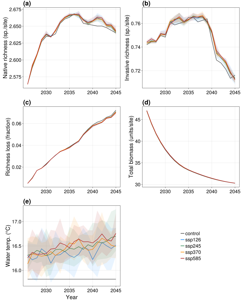
Figure 4: Annual whole-basin trajectories across emission pathways, 2026–2045. Panels: (a) native richness (species per site); (b) invasive richness (species per site); (c) realised native richness loss (fraction); (d) total biomass (model density units per site); (e) projected water temperature ( ^{\circ}\text{C} ). Lines: mean across the 11 GCMs of the whole-basin value per pathway; bands: 10–90% across GCMs. Colour: blue = SSP1-2.6, green = SSP2-4.5, orange = SSP3-7.0, red = SSP5-8.5, black = no-warming control. Temperature trajectories diverge as expected, but native richness, realised richness loss and total biomass remain nearly coincident across pathways, and the control shows a large transient decline in biomass that dominates the raw trajectories (control total biomass -35.5\% from 2026 to 2045). The temporal persistence of the pattern supports interpreting the flat aggregate climate slopes as a model result; the scenario-minus-control differences isolate the small warming signal.
