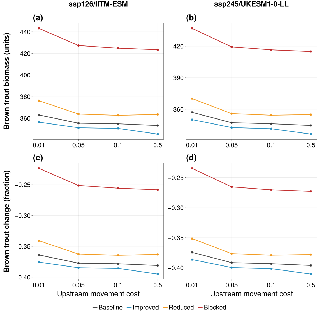
Figure 10: Brown trout response to hydraulic structure. Panels: (a) and (c) are the cool endpoint; (b) and (d) the warm endpoint. The top row is final Salmo trutta biomass and the bottom row its relative biomass change. x-axis: the four categorical upstream movement costs. Coloured lines/points: the four passability states; black = baseline, blue = improved, orange = reduced, red = blocked. Reading: all passability curves lie below the spun-up state, the warm endpoint is uniformly more negative, and at cost 0.05 the baseline-to-blocked change is 355.4 to 427.3 units at the cool endpoint (a hydraulic gain of +71.9 units), so warming and passability act on trout through different magnitudes.
