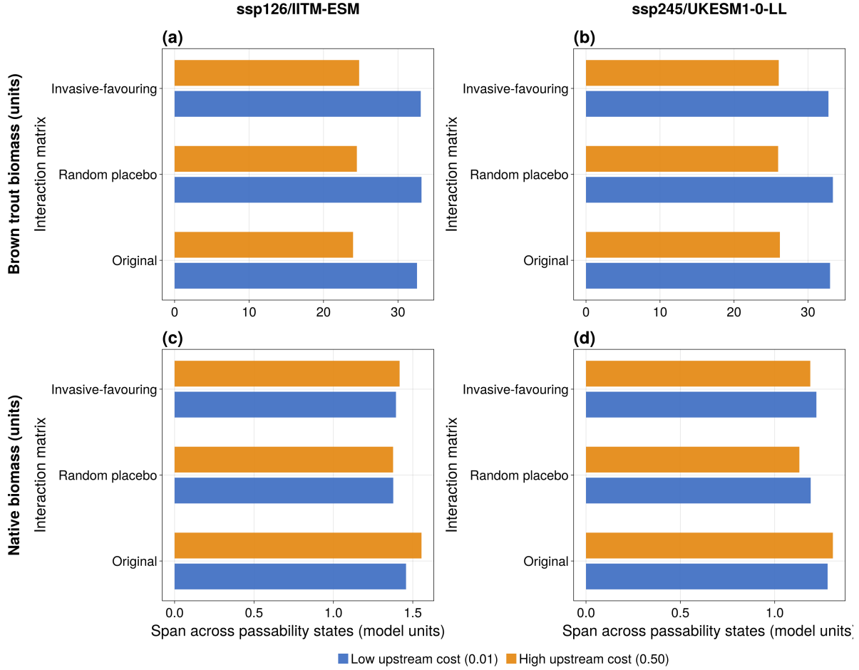
Figure 11: Passability robustness across interaction matrices. Panels: (a) and (c) are the cool climate endpoint (SSP1-2.6/IITM-ESM) and (b) and (d) the warm endpoint (SSP2-4.5/UKESM1-0-LL); the top row (a, b) is brown-trout ( Salmo trutta ) final biomass and the bottom row (c, d) basin native biomass. Axes: the y-axis lists the three interaction matrices (original, random placebo and invasive-favouring) and the x-axis is the span across passability states—the difference between the largest and smallest metric value when the four passability states (baseline, improved, reduced and blocked) are compared at the same matrix, climate endpoint and upstream cost—in model units. Bars and legend: each matrix row carries two horizontal bars, one per upstream-cost setting, and the two-colour legend printed below the panels identifies them: blue (RGBA 0.27, 0.45, 0.77) = low upstream cost (0.01) and orange (RGBA 0.90, 0.55, 0.10) = high upstream cost (0.50); these are the two colours defined in the plotting code for the cost levels 0.01 and 0.50. Reading: brown-trout spans are about 29 units and native-biomass spans about 1.3 units under every matrix and both cost settings, so the passability signal is essentially matrix-independent in the corrected sweep. This supersedes the September claim of matrix-dependent spans.
