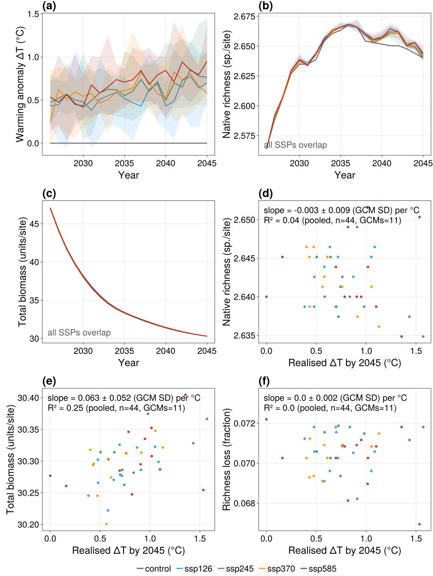
Figure 5: Forcing versus response. “Forcing” is the realised basin-mean water-temperature anomaly \Delta T relative to the 1986–2005 baseline. Top row (trajectories, median across the 11 GCMs; band = 10–90%) : (a) forcing \Delta T ( ^{\circ}\text{C} ) over time; (b) native richness; (c) total biomass, with the annotation flagging that the response trajectories lie on top of one another even though the forcing separates. Bottom row (one point per GCM \times SSP run) : (d) end-of-2045 native richness, (e) end-of-2045 total biomass and (f) end-of-2045 realised richness loss, each against the realised warming of that run. The realised anomaly is used because it is the quantity that drives the biology in each run (correction C7). Correlations are computed across the 44 scenario runs; the control is plotted for reference but excluded from the fits, matching the dose–response analysis. The loss metric is a deterministic thresholded realised loss, not an extinction probability.
