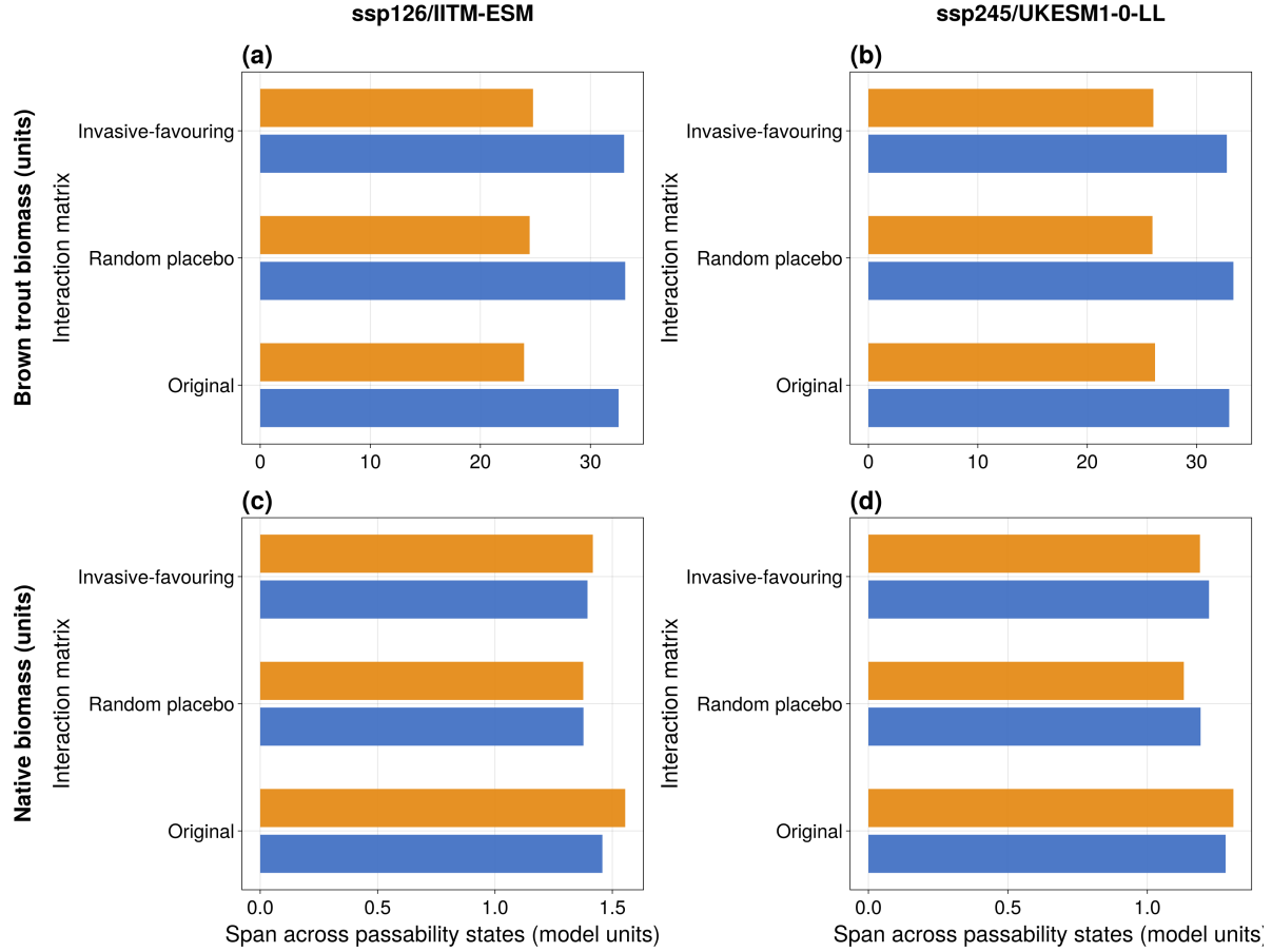
Figure 11: Passability robustness across interaction matrices. Panels: (a) and (c) are the cool endpoint; (b) and (d) the warm endpoint. The top row is brown trout final biomass and the bottom row basin native biomass. y-axis: the three interaction matrices. What each bar is: the span across passability, i.e. the difference between the largest and smallest metric value when the four passability states are compared at the same matrix, climate endpoint and cost; the two bars per matrix are the low (0.01) and high (0.50) upstream-cost settings. Reading: trout spans are about 29 units and native-biomass spans about 1.3 units under every matrix, so the passability signal is essentially matrix-independent in the corrected sweep. This supersedes the September claim of matrix-dependent spans.
