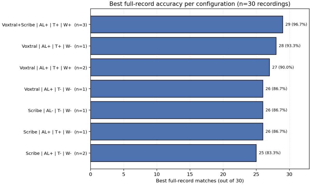
Figure 2: Best full-record matches (out of 30) per configuration. Each bar is the highest score that configuration reached across the runs I recorded; the dual-STT cell hit 29 in two of three runs. The label encodes the four design axes <STT> | <audio-LLM> | <targeted> | <Whisper>.
