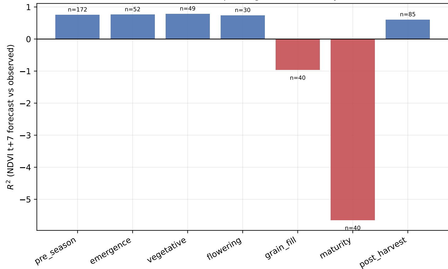
Per-phenology-stage NDVI forecast skill — EVR_01, 2025 season (senescence collapse at grain-fill / maturity)
