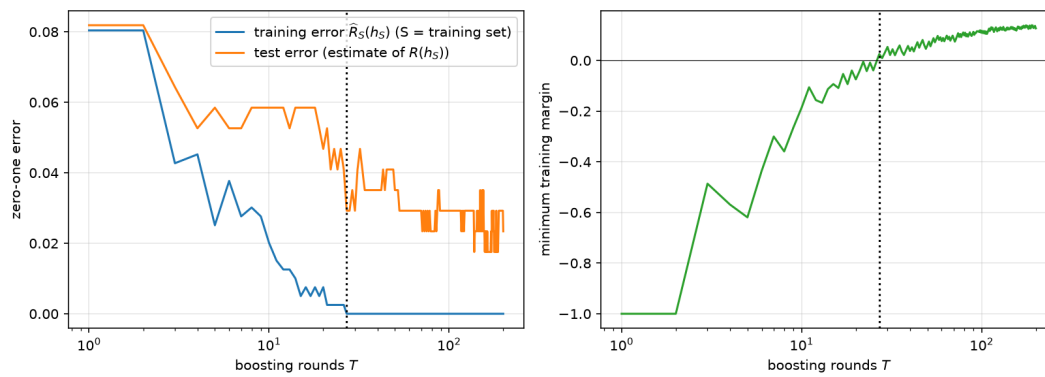
Figure 11.1: AdaBoost's training and test error (left) and minimum training margin (right) as a function of the number of boosting rounds T , on a logarithmic axis; the dotted line marks the round at which training error first reaches zero.
