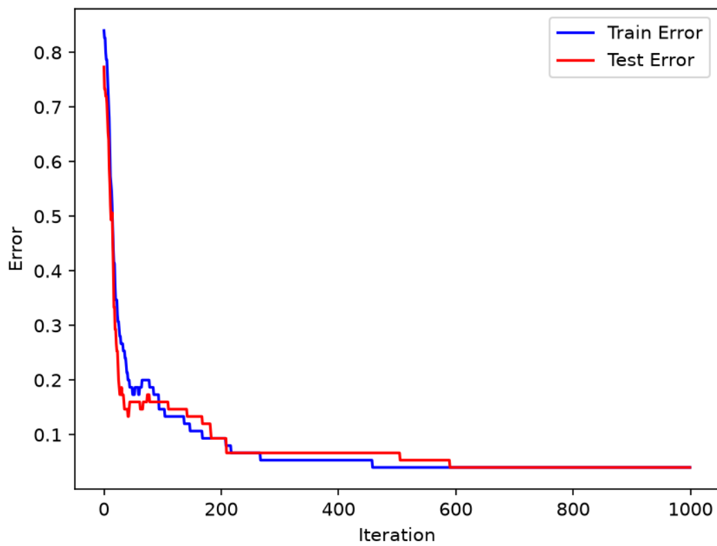
Figure 3.1: Training and test error of the generative linear classifier across gradient descent iterations.
