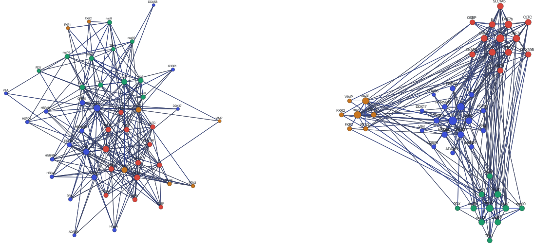
Fig. 3. The same network under the two arrangements that answer different questions: SARS-CoV-2 in release 5.0.260 at trust \geq 0.4 , keeping proteins with at least two partners and the best-supported 248 interactions — 48 proteins. Colour is the trust-weighted community. Left , force: what clusters together. Right , grouped: the 4 communities as packed discs. The communities are not told any biology, and correspond to it anyway — the replication-transcription complex (nsp5, nsp7–nsp16) in green; the membrane and ER proteins M, E, ORF6, ORF7a/b and nsp6 with host VAPB, OSBP, CLTC and CKAP4 in red; nsp3 and nsp4 with the reticulons RTN3 and RTN4 in orange; N and S with host chaperones and RNA-binding proteins in blue.
